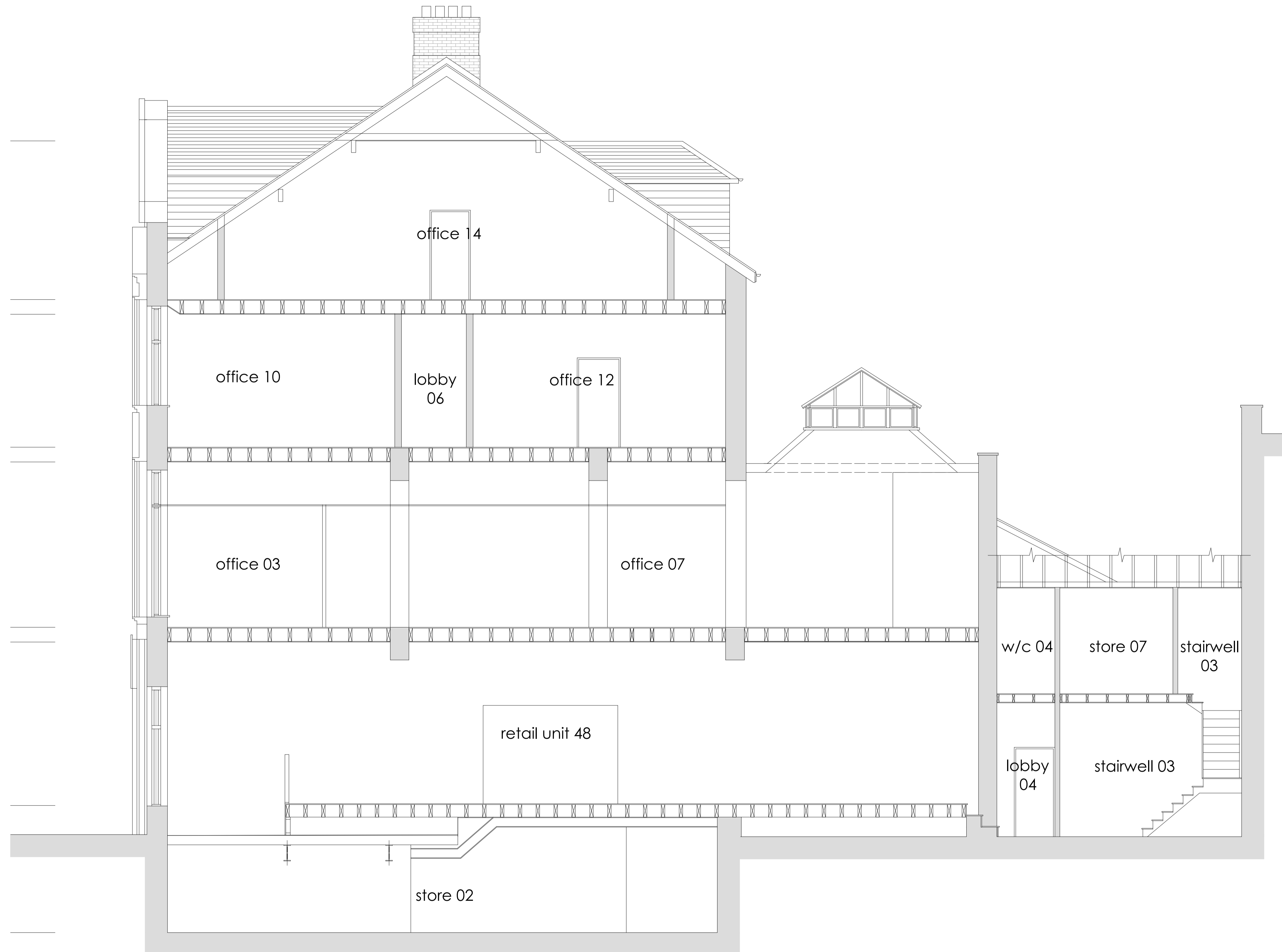
section b-b
